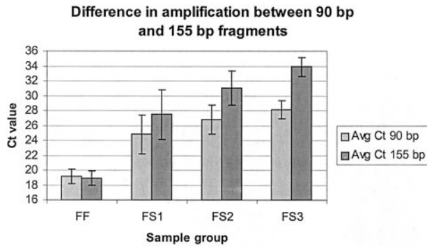
Figure 1. Real-time PCR analysis of RNAs isolated from FFPE tissues with different duration of storage. The Ct values (y axis) for two amplicons of different sizes that monitor a highly expressed gene, RPL13A, were plotted for each sample group (x axis): FF, fresh-frozen; FS1, 1 year; FS2, 2 years; FS3, 9–11 years. The average difference in the Ct values ( \Delta Ct) of the two amplicons was derived from each sample group as -0.3 \pm 0.1 , 2.7 \pm 1.1 , 4.2 \pm 1.1 , and 5.8 \pm 1.0 , respectively. The error bars represent the SD from the mean.
